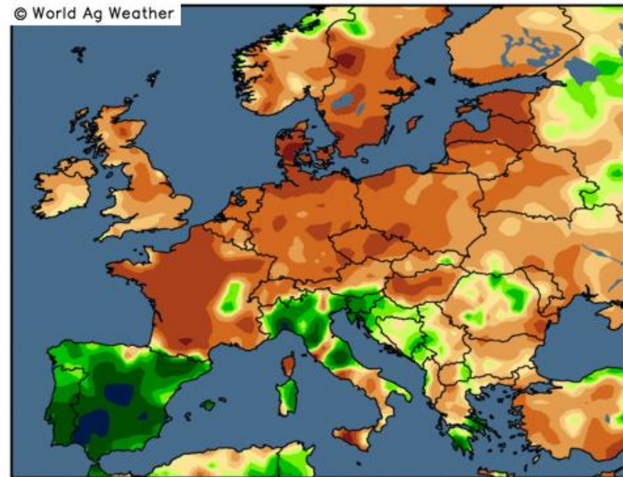
90-day Precipitation Analysis Percent of normal through 16 Apr 2025
